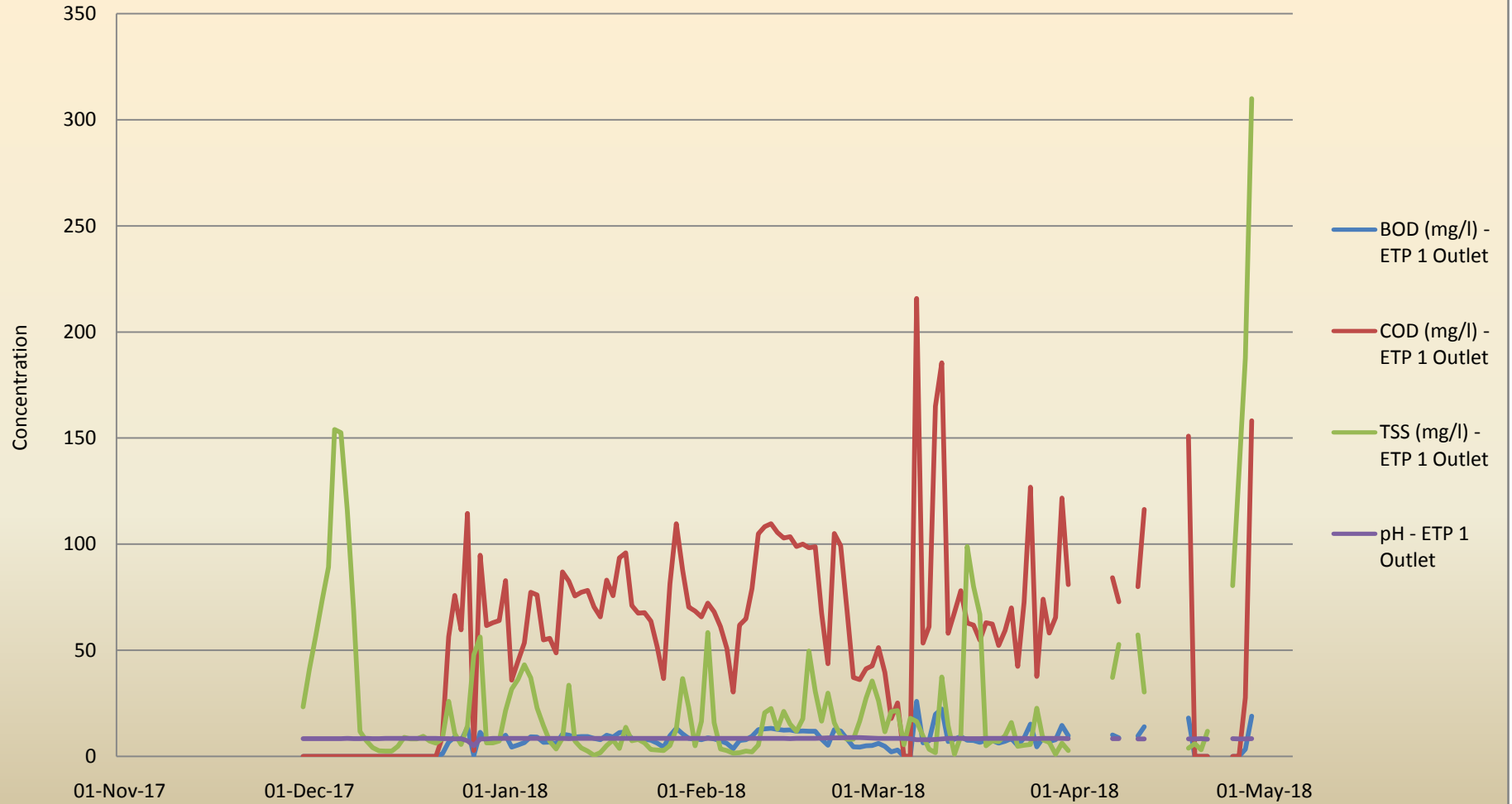
Effluent Trend (2017-18) in M/s. Reva Kripa Sugar (P) Ltd., Dist. Jabalpur (M.P.)
